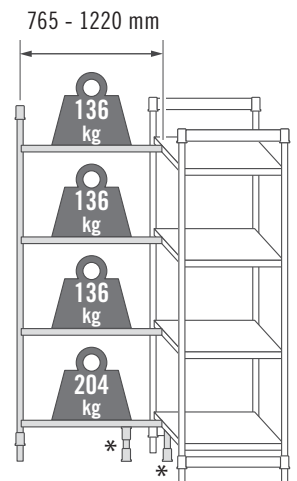
Corner Unit with 2 Dunnage Stands
