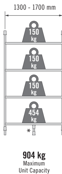
Single Unit with Dunnage Stand
